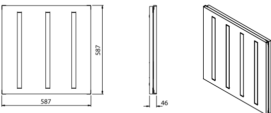
60x60 Sasled Surface Mounted (3-4 Bar) Luminaire
